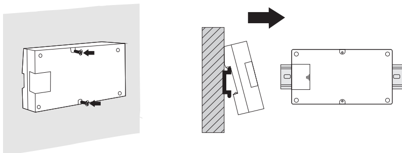
Direct wall-mounted
